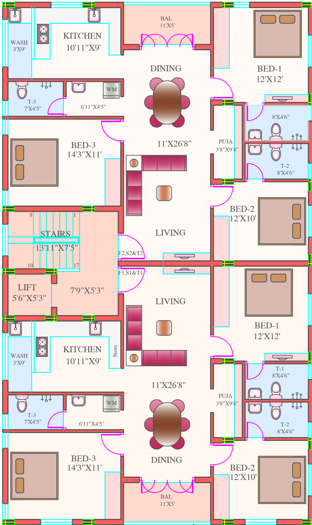
FIRST , SECOND & THIRD FLOOR PLAN
